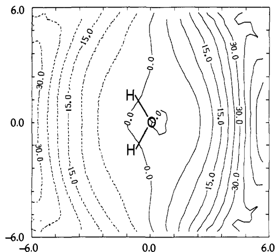
Figure 4. Contours of the relative difference in the electron density of water between isolated conditions and perturbation by an electric field along the symmetry axis of 0.01 \text{ au} ( 5.14 \times 10^7 \text{ V/cm} ). Difference contours are in percent of the density of isolated water and are drawn for the plane of the molecule.
